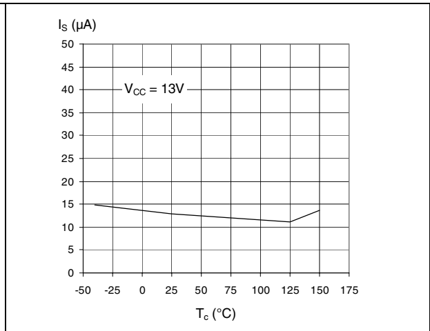
Figure 9. Off state supply current
