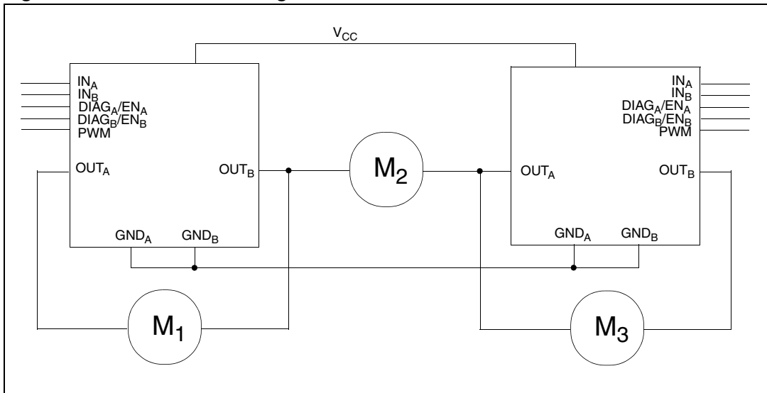
Figure 34. Multi-motors configuration
